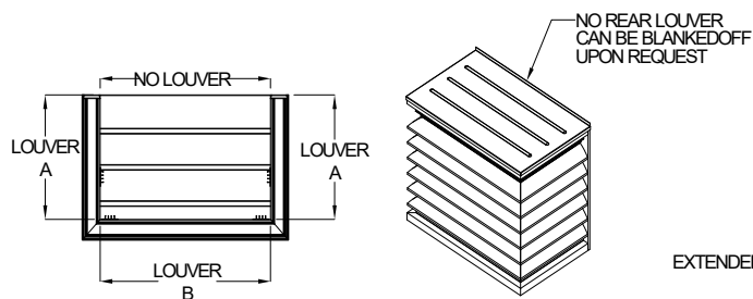
3 SIDED PENTHOUSE
