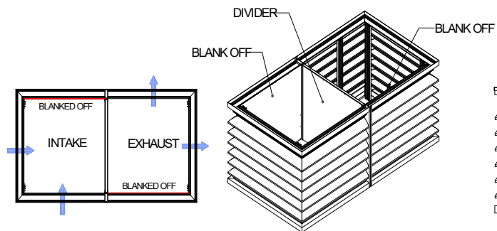
DIVIDER / BAFFLE
