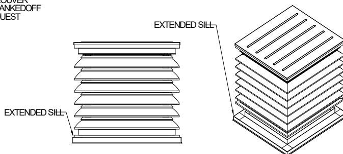
EXTENDED SILL / NO FLANGE BOTTOM
